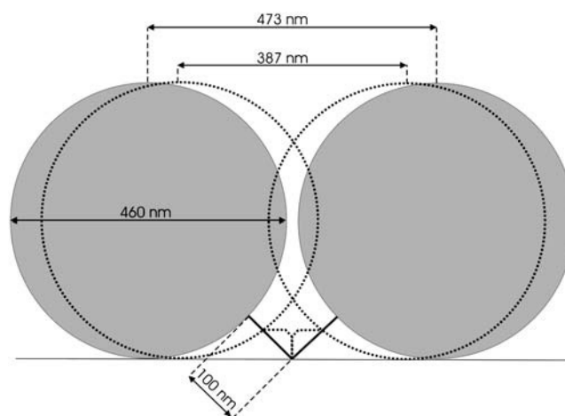
FIGURE 1 Scale-drawing of 0.46 \mu\text{m} bead tethered to surface by 324 bp of DNA, side view. The full-line circles illustrate the extremal positions the bead can take when the DNA is straight. The dashed-line circles show the extremal positions the bead can take when the DNA is modeled as two stiff rods at right angles to each other. The difference between the positions of the center of the bead at the two extrema is nearly 100 nm. The Brownian RMSD is a measure for the variance in the bead's x,y -positions. Thus, the change in Brownian RMSD upon bending of the DNA will be less than the change in extremal positions.
