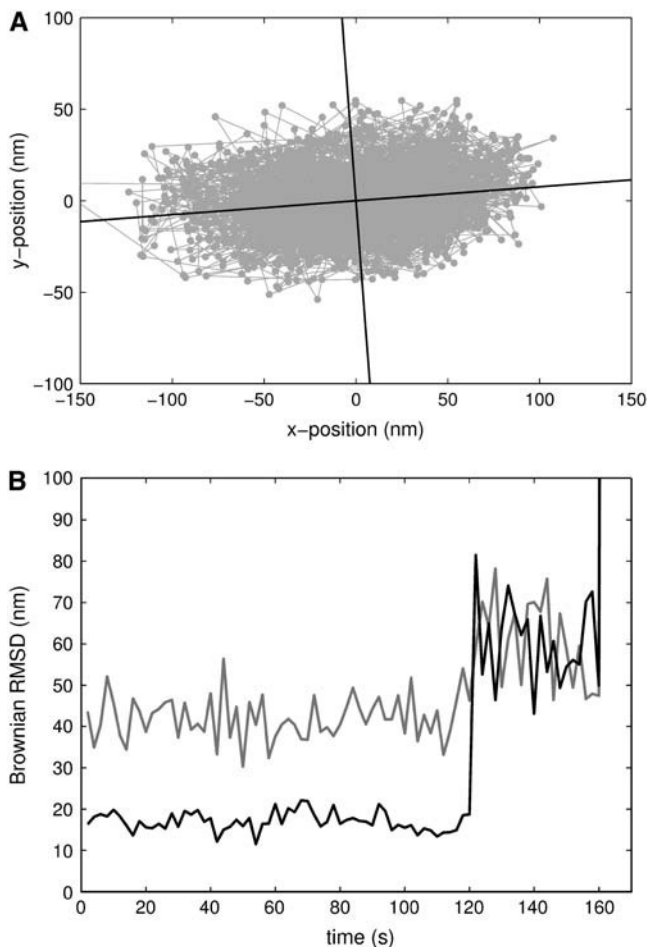
FIGURE 6 Time-series of Brownian motion for a 1\text{-}\mu\text{m} diameter silica bead tethered by control-DNA, in the presence of Xho I. (A) Scatter-plot showing principal axes. (B) The square-root of the two principal moments, \sqrt{I_{\max}} and \sqrt{I_{\min}} , are shown in shaded and solid representations, respectively. During the first 120 s, the motion of the bead was highly anisotropic (isotropy measure, r = 39\% ). After 120 s, the motion of the bead was isotropic ( r = 94\% ); the bead released from the surface after 160 s.
