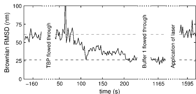
FIGURE 7 Time-evolution of Brownian RMSD (calculated in nonoverlapping 2-s windows) during laser-tweezers experiment. The stepwise binding of TBP to DNA started \sim 80\text{ s} after 30\text{ }\mu\text{l} 226\text{ nM} TBP was flowed in. Approximately 20 min after addition and binding of TBP, the tweezers were used to pull the silica bead horizontally, thus stretching the tether. After this stretching, B returned to its original value, suggesting that the protein was forced off the DNA.
